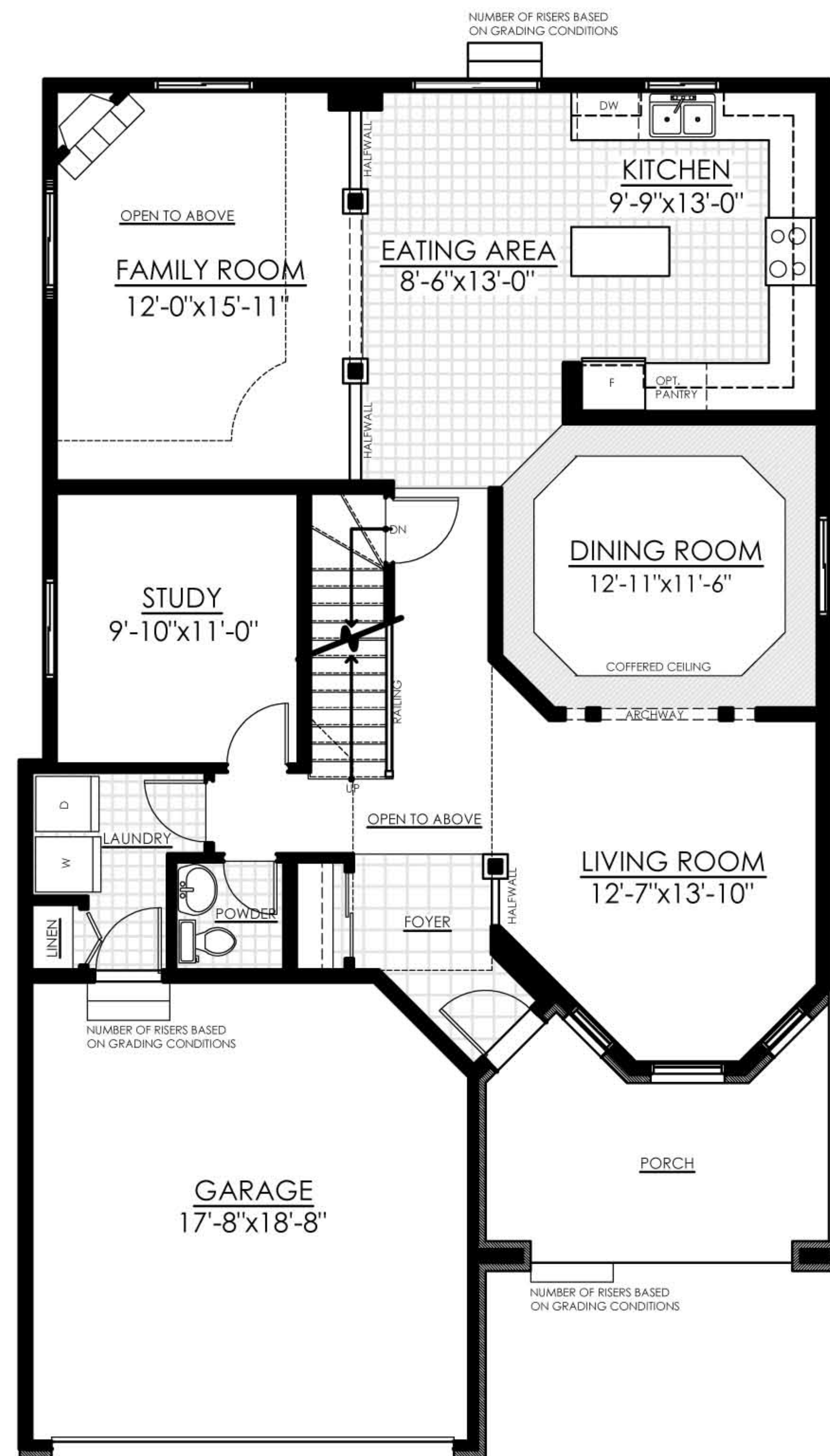
Ground Floor GROUND FLOOR PLAN
